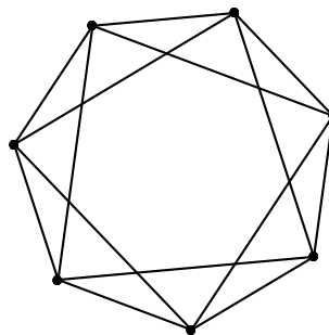
Figure 6: The square of a circle C_7^2
