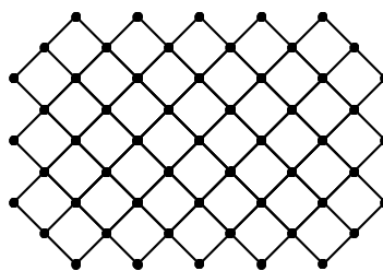
Figure 11: The odd Aztec rectangle OR_{5,3}
