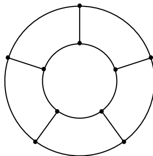
Figure 8: The cyclic ladder K_2 \oplus C_5
