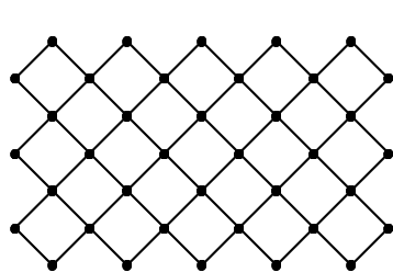
Figure 10: The even Aztec rectangle ER_{5,3}
