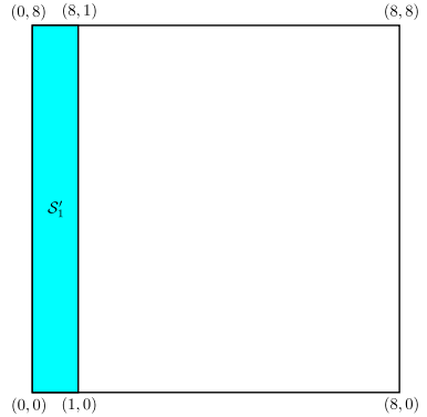
Figure 2: The strip \mathcal{S}'_1 \subseteq \mathbb{T}^2 .
