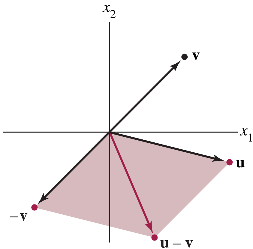
FIGURE 7 Vector subtraction.
