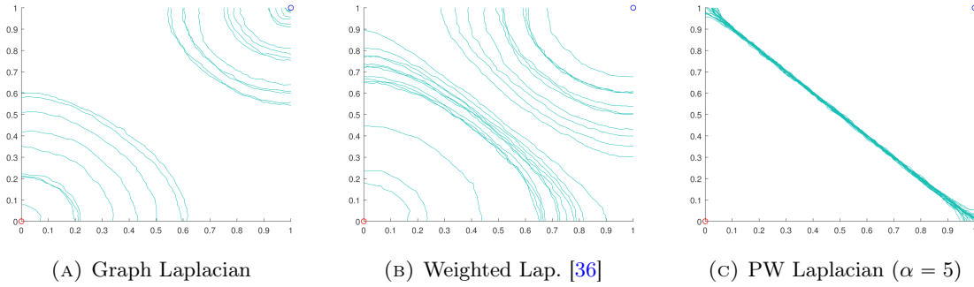
FIGURE 4. Comparison of decision boundaries plotted over 25 random trials for a synthetic classification problem for (A) the standard graph Laplacian, (B) the nonlocal graph Laplacian [36], and (C) our properly-weighted graph Laplacian. Two labels are given, g(0,0) = 0 (red point) and g(1,1) = 1 (blue point), and the graph is a uniform random geometric graph (described in the text).
