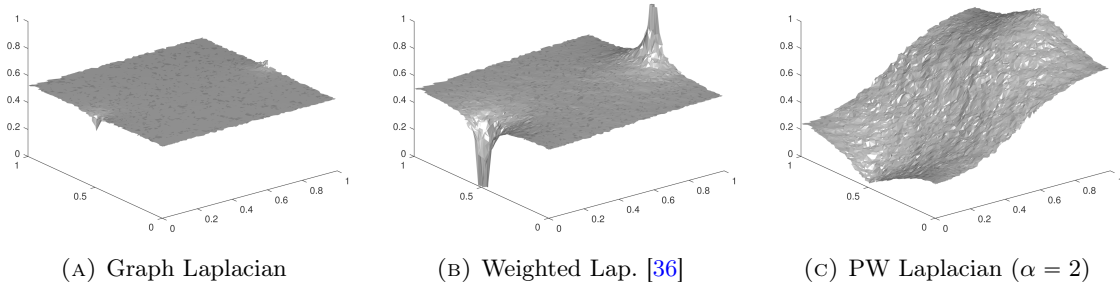
FIGURE 3. Comparison of (a) the standard graph Laplacian, (b) the nonlocal graph Laplacian [36], and (c) our properly-weighted Laplacian. The graph is a random geometric graph (described in the text) on [0, 1]^3 , and the surfaces plotted are a slice of the learned function u near x_3 = 0.5 . The labels are g(0, 0.5, 0.5) = 0 and g(1, 0.5, 0.5) = 1 .
