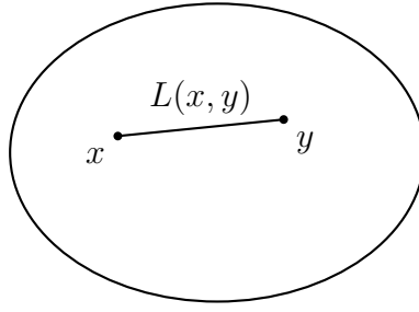
Convex Set
