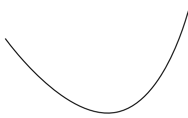
Convex Function
