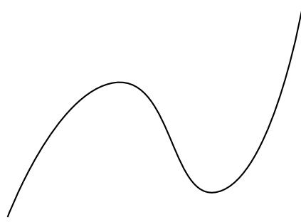
Non-Convex Function
