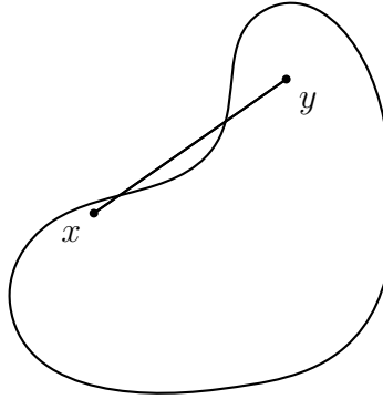
Non-Convex Set
