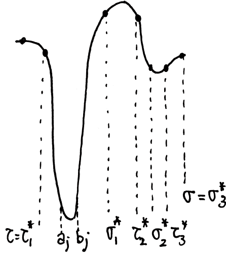
Figure 2: A function u_\varepsilon and the related [\tau^*, \sigma^*] subdivision
