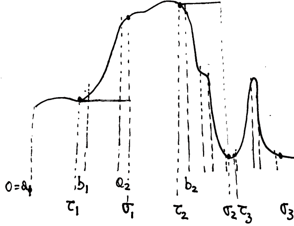
Figure 1: A function u_\varepsilon and the related [\tau, \sigma] subdivision
