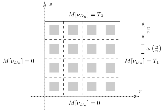
FIGURE 5.1. The situation in Lemma 5.1.
