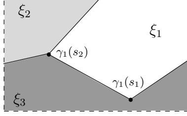
FIGURE 1.2. If we chose \xi_1, \xi_2, \xi_3 so that \zeta_1 is continuous at the corner point \gamma_1(s_1) and it jumps at \gamma_1(s_2) , then condition (1.16) is imposed at \gamma_1(s_1) , while condition (1.14) is imposed at \gamma_1(s_2) .
