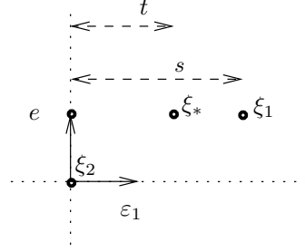
FIGURE 6.3. The mutual positions of the colors in u .
