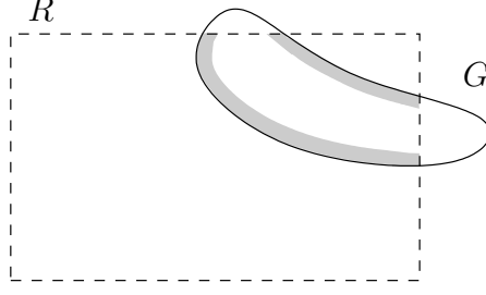
FIGURE 5.3. The situation in Lemma 5.2. The region R \cap G^\delta is colored in gray.
