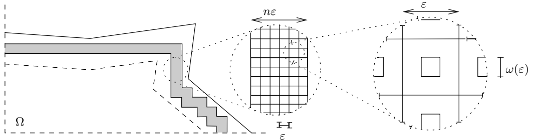
FIGURE 5.5. The construction in Step 3. The set D_{k, \varepsilon} is represented in the picture as the set \Sigma(\delta) \cap \Omega after removing the colored squares contained in the shaded region.
