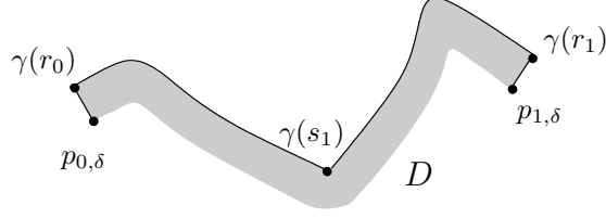
FIGURE 4.2. The situation in Lemma 4.3.
