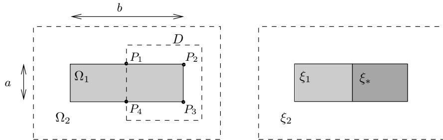
FIGURE 6.5. The situation in Example 6.3.
