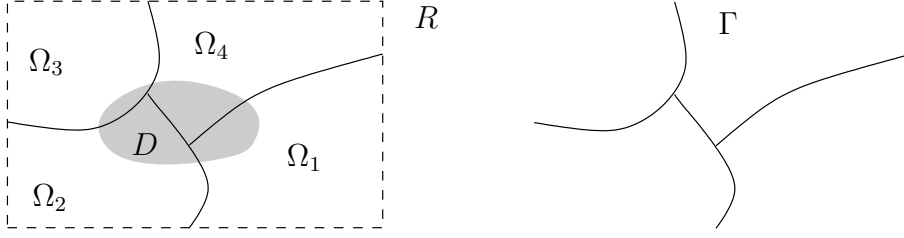
FIGURE 1.1. An admissible image u_0 , with its contour \Gamma and a damaged region D .
