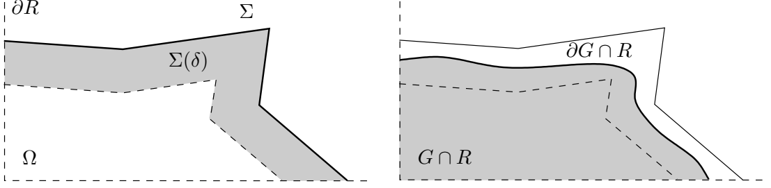
FIGURE 5.4. On the left, the sets \Omega , \Sigma and \Sigma(\delta) \cap \Omega . On the right, the sets G \cap R and \partial G \cap R .
