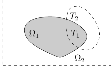
FIGURE 6.2. The dashed line is the contour of the damaged region D .
