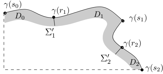
FIGURE 4.4. The field M is obtained by gluing together the constructions of Lemma 4.3 performed on each D_i .
