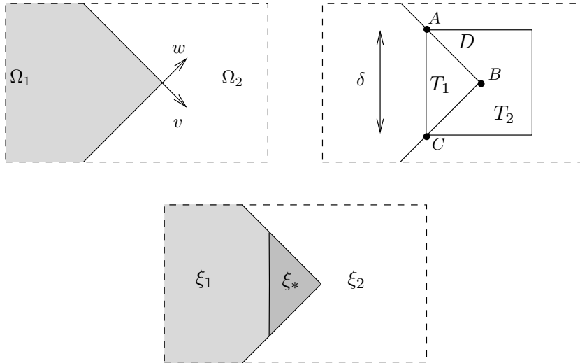
FIGURE 6.4. The situation in Example 6.2. Since |z_{12}| > 1/\sqrt{2} , the minimizer u over the damaged region D is different from u_0 and presents a new contour, no matter how small the side length of D .
