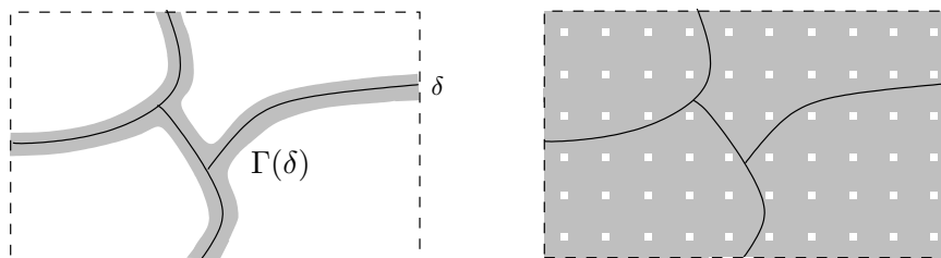
FIGURE 1.3. On the left figure, \Gamma(\delta) is a neighborhood of width \delta of the contour \Gamma of u_0 \in \text{Ad}(R) . On the right figure, the color is given only inside small and uniformly distributed squares. Note that here the damaged region contains a small neighborhood of the contour \Gamma .
