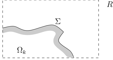
FIGURE 4.3. The shaded region is \Sigma(\delta) \cap \Omega_k .
