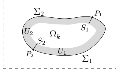
FIGURE 4.1. The case in which \Sigma is a closed curve.
