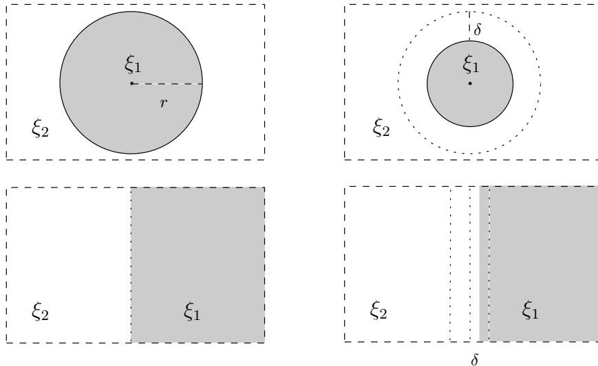
FIGURE 6.1. Example 6.1: in the first picture u_0 is not a minimizer, in the second one there is lack of uniqueness. In both cases the compatibility vector \zeta between \xi_1 and \xi_2 is a unit vector.
