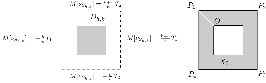
FIGURE 5.2. Construction of M , and the set X .
