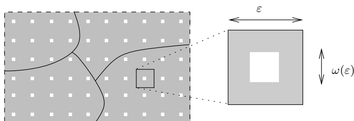
FIGURE 1.4. An example of an \varepsilon -uniformly distributed (undamaged) region.
