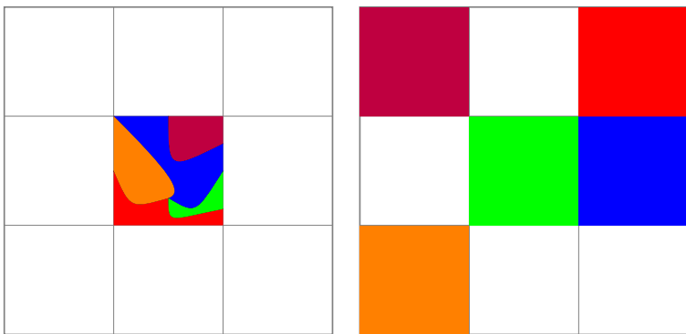
FIGURE 1. One example of an expanding Bernoulli map \varphi . The colored regions on the left are mapped to regions of the same color on the right.
