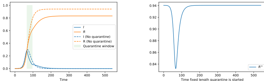
FIGURE 2. Left: I, R vs t both with a 30 day, optimally scheduled, quarantine and without any quarantine. Right: The value of R(\infty) vs the time when a 30 day quarantine is started.
