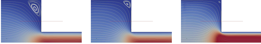
FIG. 6.2. Contraction flow for We = 1, 10, and 100 (streamlines over velocity magnitude).
