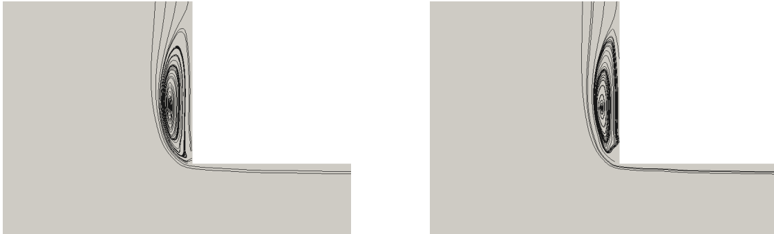
FIG. 6.7. 4:1 Contraction with We = 5 and We = 10 .
