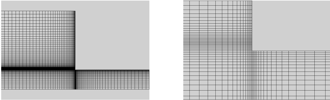
FIG. 6.4. Mesh and refinement near the reentrant corner, 4200 elements.
