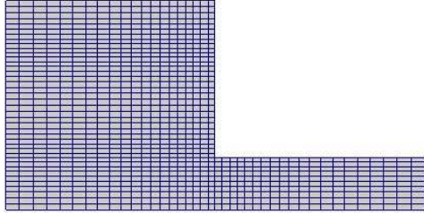
FIG. 6.3. Mesh and data for solutions in Figure 6.1.
