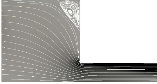
FIG. 6.5. Typical streamlines and numerical and rheological data for lip vortex calculations
