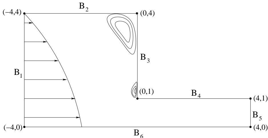
FIG. 6.1. Geometry of 4:1 Contraction
