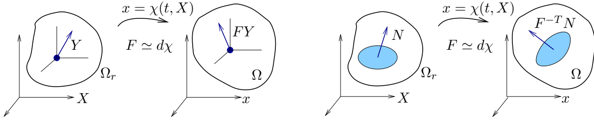
FIG. 2.1. Transport of a fiber (left) and loop or disk (right).
