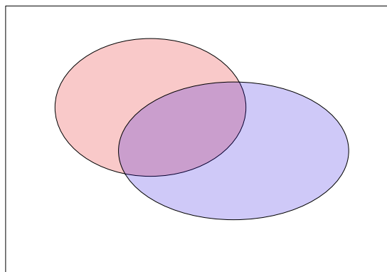
Figure 1: Imagine that the rectangle describes the possible universe \Omega . If A is the red set, and B is the blue set, then the purplish set where the two overlap is A \cap B . The set A \cup B is all colored portions of the diagram.
