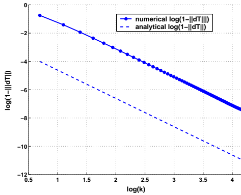
Figure 2.5. Convergence factor of Lloyd method for \rho(x) = e^{-x^2} .
