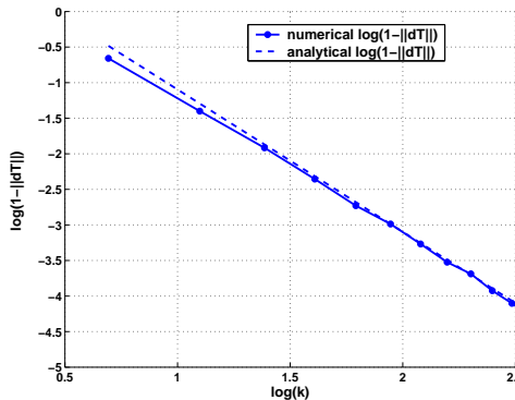
Figure 2.6. Convergence factor of Lloyd method for \rho(x) = 1 + x^4 \cos(\pi x) .
