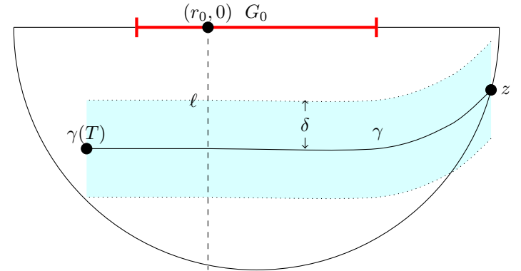
FIGURE 4. The curve \gamma starts on \partial B(0, \varepsilon^2) , goes through the line \ell while keeping a distance \delta from the gate G_0 .
