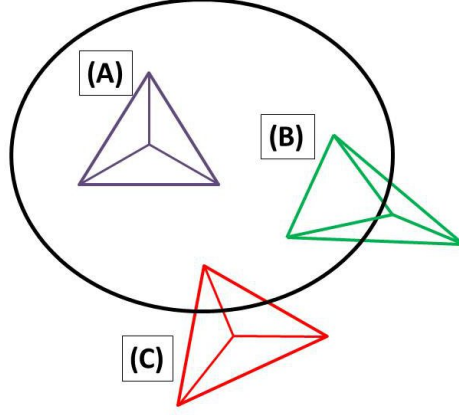
Fig. 2: Coupling used in Lemma 7.
