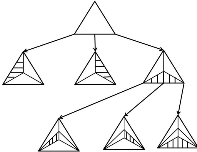
Fig. 4: RANs as random ternary trees.
