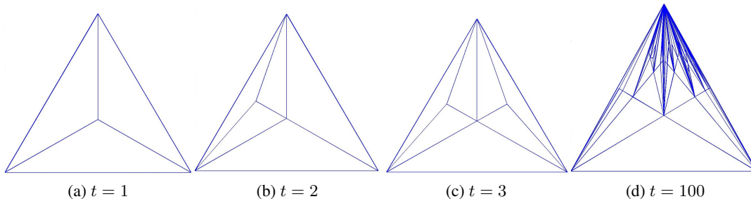
Fig. 1: Snapshots of a Random Apollonian Network (RAN) at: (a) t = 1 (b) t = 2 (c) t = 3 (d) t = 100 .
