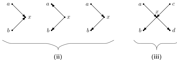
Figure 2: Properties (ii) and (iii) of digraph (\epsilon, p) -regularity. The number of such vertices, x , should be approximately what it is in the random digraph D_{\nu, p} .
