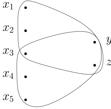
Figure 1: An example with k = 5 , \ell = 2 , d = 2 and s = 2 with A_1 = \{x_1, x_2, x_3\} , A_2 = \{x_3, x_4, x_5\}
