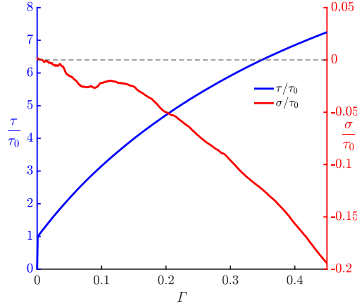
Figure 17: Normal and transverse reaction stress on the top boundary of the free-standing film subjected to simple shearing, for H = 0.5 \mu m .
