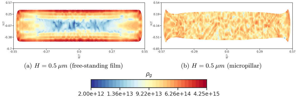
Figure 8: \rho_g = |\boldsymbol{\alpha}|/b ( m^{-2} ) at |e_m| = 15\% in the metal film for the free-standing film and the micropillar sandwich with 90^\circ orientation. The corresponding |e| for the micropillar is 1.56%.
