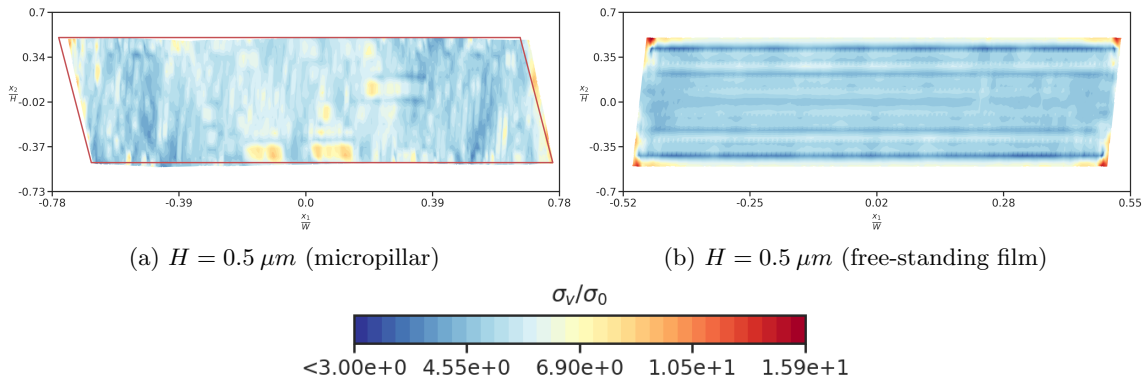
Figure 15: von Mises stress at \Gamma_m = 30\% in the metal film for the micropillar sandwich with 45^\circ orientation and for the free-standing film. The corresponding |e| for the micropillar is 1.15%, and the solid red line in (a) shows the boundary of the undeformed metal thin film.
