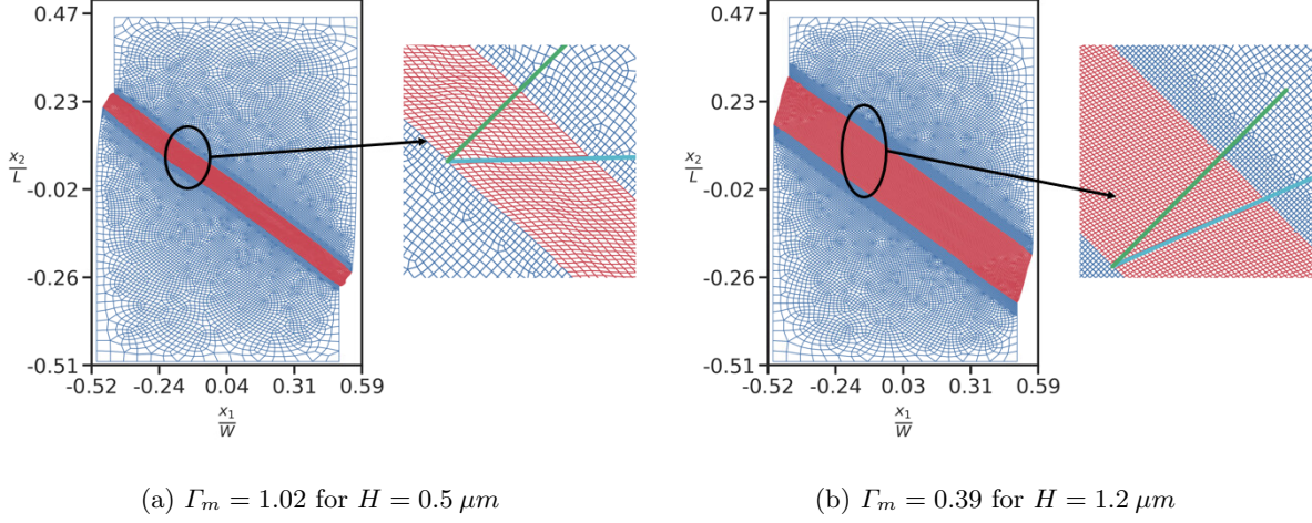
Figure 11: Nominal shear strain ( \Gamma_m ) in the film at |e| = 3.5\% for micropillar with 45^\circ orientation, for different film thickness ( H ). The green solid line denotes an undeformed line, while the cyan solid line denotes the corresponding deformed line.
