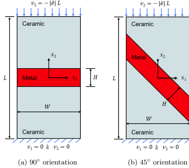
Figure 2: Schematic of idealized plane strain model of micropillar compression experiments.
