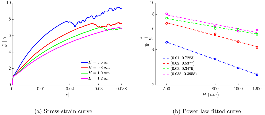
Figure 7: (a) Stress-strain response in compression of the micropillar sandwich with 45^\circ orientation and for different film thickness ( H ). (b) Power law fitted for the stress vs film thickness ( (\tau - g_0)/g_0 = a H^m ) at 1% – 3.5% strain. The first and second term in the legend denote the strain and magnitude of power law exponent ( |m| ), respectively.
