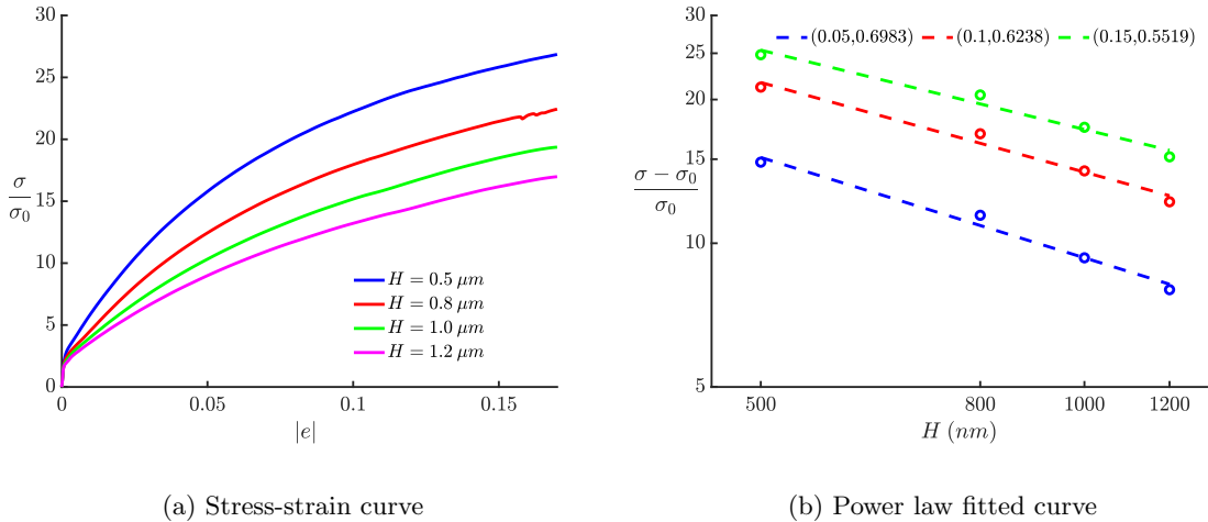
Figure 4: (a) Stress-strain curve in compression of the free-standing film for different film thickness ( H ). (b) Power law fitted for the stress vs film thickness ( (\sigma - \sigma_0)/\sigma_0 = a H^m ) at 5% – 15% strain. The first and second term in the legend denote the strain and magnitude of power law exponent ( |m| ), respectively.
