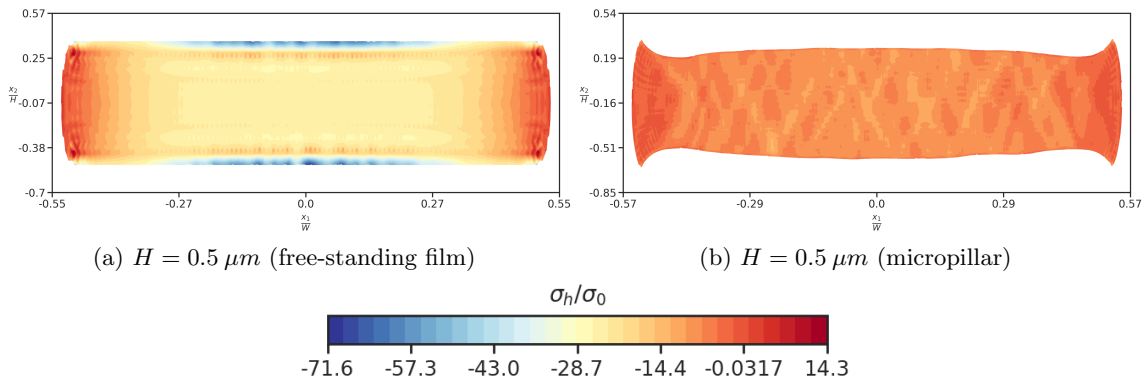
Figure 10: Hydrostatic stress at |e_m| = 15\% in the metal film for the free-standing film and the micropillar sandwich with 90^\circ orientation. The corresponding |e| for the micropillar is 1.56%.
