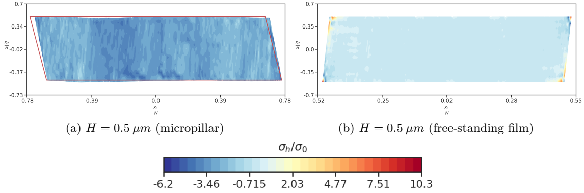
Figure 16: Hydrostatic stress at \Gamma_m = 30\% in the metal film for the micropillar sandwich with 45^\circ orientation and for the free-standing film. The corresponding |e| for the micropillar is 1.15\% , and the solid red line in (a) shows the boundary of the undeformed metal thin film.
