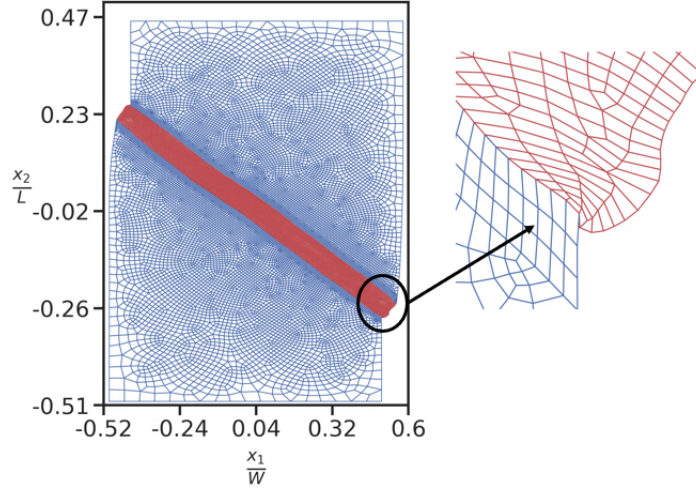
Figure 12: The deformed mesh for the micropillar with 45^\circ orientation for H = 0.5 \mu m at |e| = 3.8\% , when the film material is close to penetrating into ceramic blocks.
