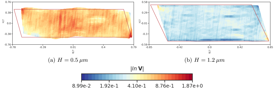
Figure 13: Norm of Logarithmic strain tensor ( |\ln(\mathbf{V})| ) at 3.5% compression strain in the micropillar sandwich with 45^\circ orientation, for different film thickness ( H ). The solid red line shows the boundary of the undeformed metal thin film.
