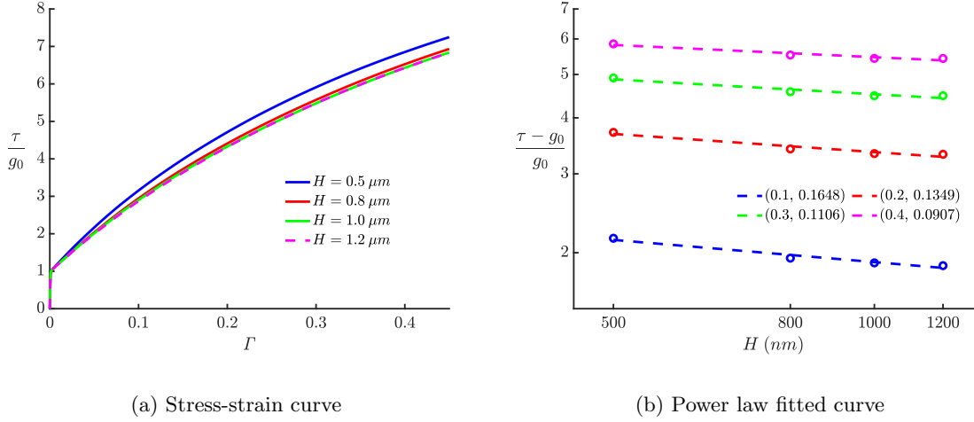
Figure 3: (a) Stress-strain curve in simple shear of the free-standing film for different film thickness ( H ). (b) Power law fitted for the stress vs film thickness ( (\tau - g_0)/g_0 = a H^m ) at 10% – 40% strain. The first and second term in the legend denote the strain and magnitude of power law exponent ( |m| ), respectively.
