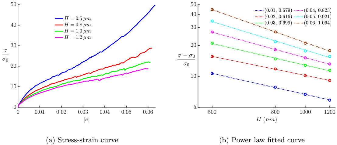
Figure 5: (a) Stress-strain curve in compression of the micropillar sandwich with 90^\circ film orientation and for different film thickness ( H ). (b) Power law fitted for the stress vs film thickness ( (\sigma - \sigma_0)/\sigma_0 = aH^m ) at 1% – 6% strain. The first and second term in the legend denote the strain and magnitude of power law exponent ( |m| ), respectively.
