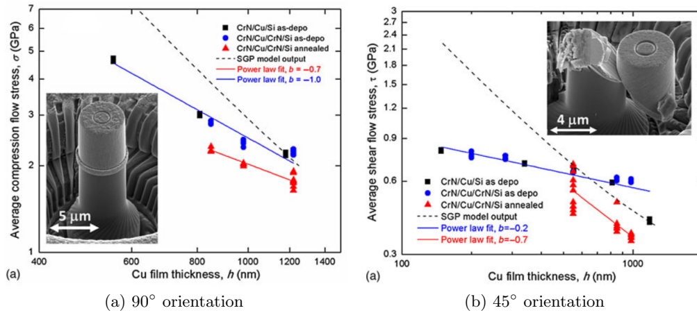
Figure 1: Micropillar experimental specimen and size effect results in both 90° and 45° orientations (Figures reprinted from [MZHM16] with permission from Springer Nature ).
