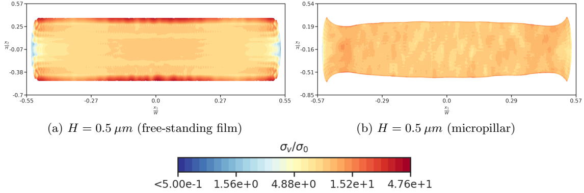
Figure 9: von Mises stress at |e_m| = 15\% in the metal film for the free-standing film and the micropillar sandwich with 90^\circ orientation. The corresponding |e| for the micropillar is 1.56%.
