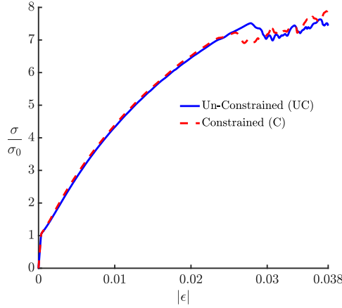
Figure 18: Stress-strain curve for the micropillar sandwich with 45^\circ orientation for H = 0.8 \mu m case and with C and UC metal-ceramic interface.
