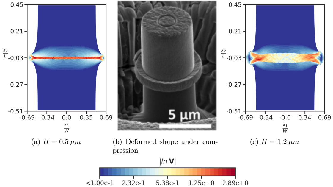
Figure 6: Norm of Logarithmic strain tensor ( |\ln(\mathbf{V})| ) at 6% compression strain ( |e| ) for the micropillar sandwich with 90^\circ film orientation for different film thickness ( H ), and comparison of the deformed shape with the experimental results [ZZM + 17]. (Figure in (b) reprinted from [ZZM + 17] with permission from Elsevier ).
