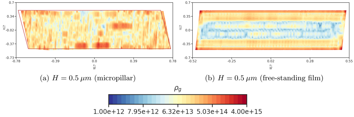
Figure 14: \rho_g = |\alpha|/b ( m^{-2} ) at \Gamma_m = 30\% in the metal film for the micropillar sandwich with 45^\circ orientation and for the free-standing film. The corresponding |e| for the micropillar is 1.15%, and the solid red line in (a) shows the boundary of the undeformed metal thin film.
