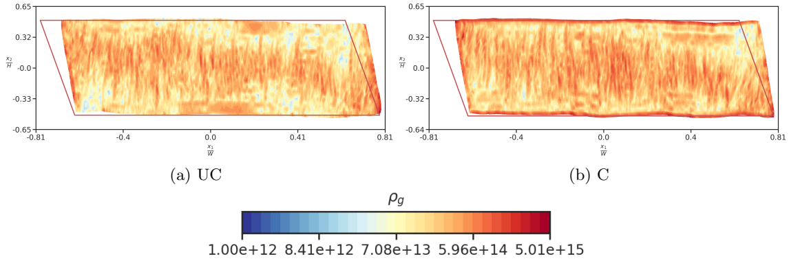
Figure 19: \rho_g = |\alpha|/b (m^{-2}) at |e| = 3.5\% for H = 0.8 \mu m with C and UC metal-ceramic interface. The solid red line shows the boundary of the undeformed metal thin film.
