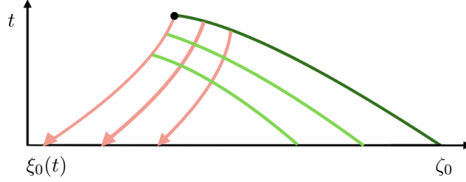
FIGURE 1. Pullback from - characteristics along + characteristics. “•” marks the point (x, t) where x = X_+(\xi_0(t), t) = X_-(\zeta_0, t) .
