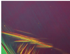
Solid-solid transformation
