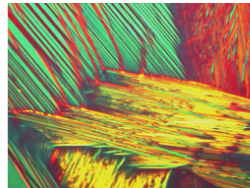
Martensite variants
