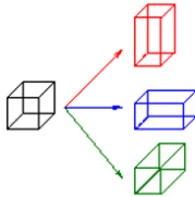
Solid-solid transformation
