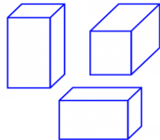
Martensite variants
