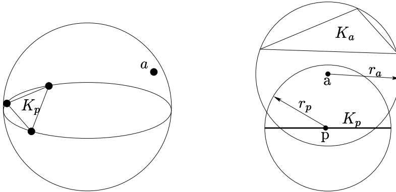
Figure 13: (a) 3d circumcenter encroaching a facet, (b) 2d circumcenter encroaching a segment.
